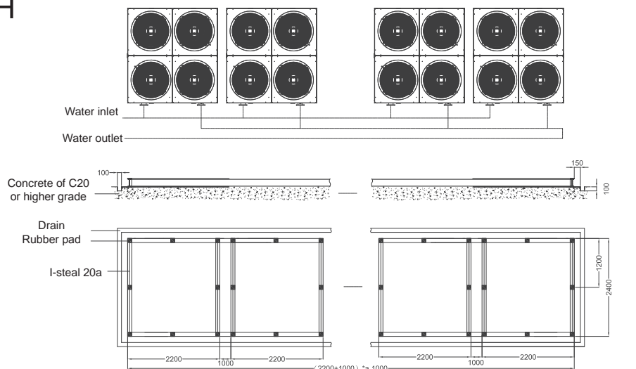
1. I-steel foundation diagram
