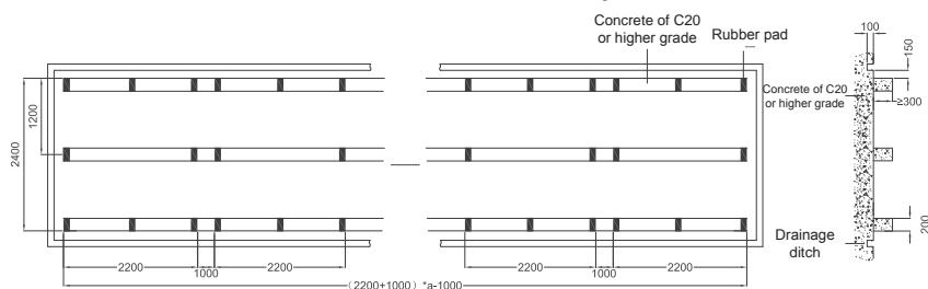
2. Concrete foundation diagram
