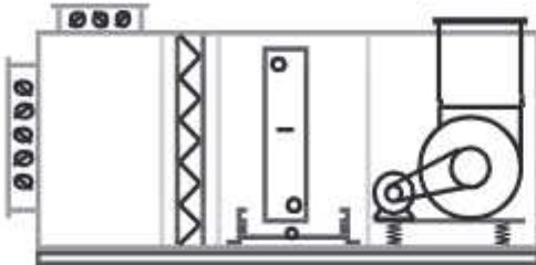
Mixing + Panel Filter + Cooling Coil + Fan
