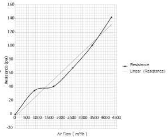
F7 Bag Filter ( 24''x24'' )
