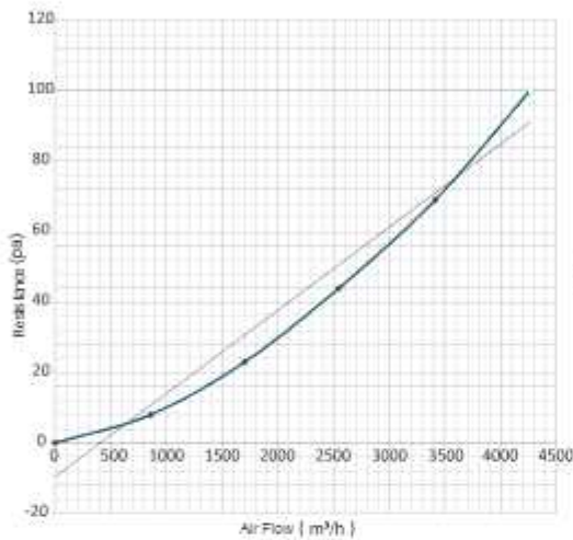
G4 Plate Filter ( 24''x24'' )
